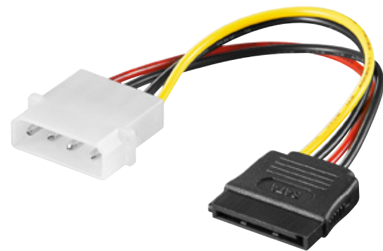
Goobay PC power cable/adapter; 5.25 inch male to SATA 4-pin 5.25 inch power plug > 15-pin S-ATA
