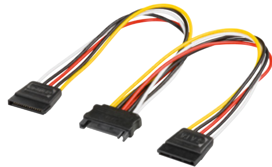
Goobay PC Y power cable/adapter; SATA 1x male to 2x female 2 SATA-Standard male > SATA Standard female
